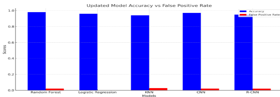
Fig. 3. False Positive Graph of different model
